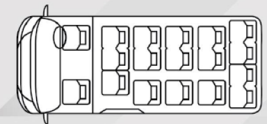
18 Seat Layout
